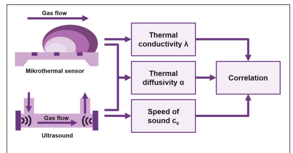
Measurement principles and their measured physical properties Own presentation
