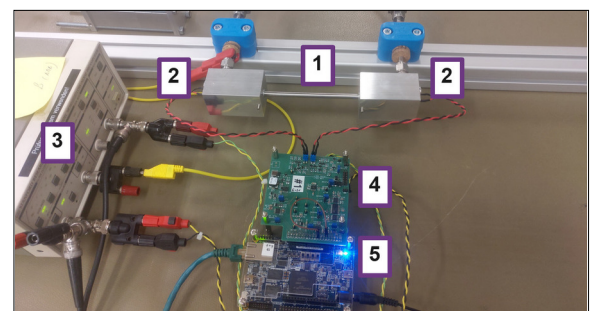
Laboratory setup ultrasound (1 Measurement tube, 2 Transducers, 3 Amplifier, 4 Analog front end, 5 Data acquisition) Own presentation
