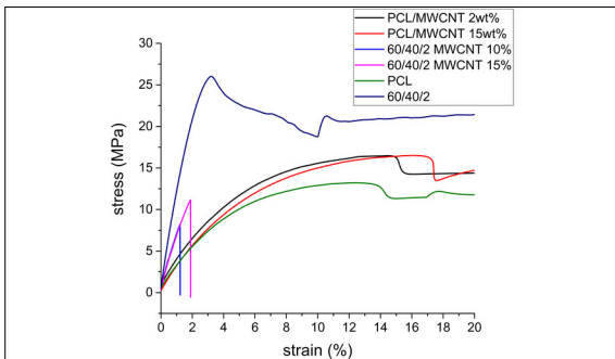
influence of MWCNT filler content on mechanical properties of neat PCL and PLA/PCL blend
