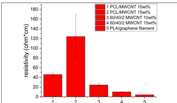
electrical resistivity of processed composite strings measured with 4 point-probe measurement (with a current of 1 mA)
